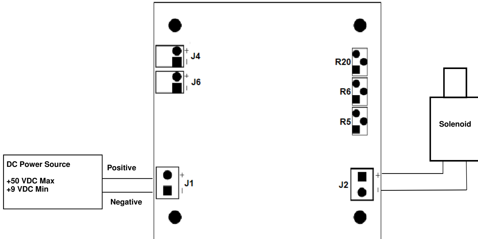
LOC - 01 Wiring Diagram
